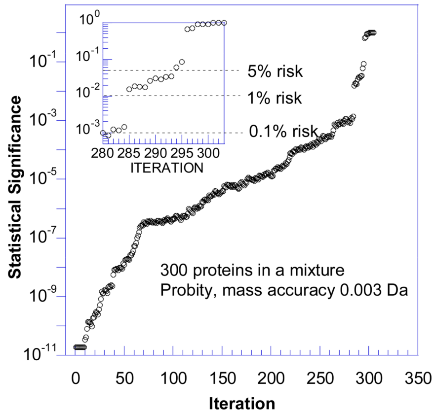
Figure 2. The statistical significance of proteins identified by peptide mass fingerprinting in a mixture of 300 proteins using an iterative method. The inset displays a magnified portion of the graph for the 280th to the 300th protein identified (Source: Reference 13).
