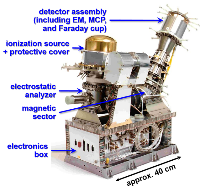
FIGURE 4 The analyzer module of the double focusing mass spectrometer (DFMS) instrument, part of the Rosetta Orbiter Sensor for Ion and Neutral Analysis (ROSINA) experiment onboard the Rosetta spacecraft, consists of high- and low-resolution entrance slits, an electrostatic analyzer followed by a magnetic sector, and a suite of “zoom” ion optics that together enable the instrument to achieve a mass resolving power higher than previous sector field mass spectrometer (SFMS) spaceflight instruments. Three distinct detectors support a 10^{10} total dynamic range. Image courtesy of the University of Bern
