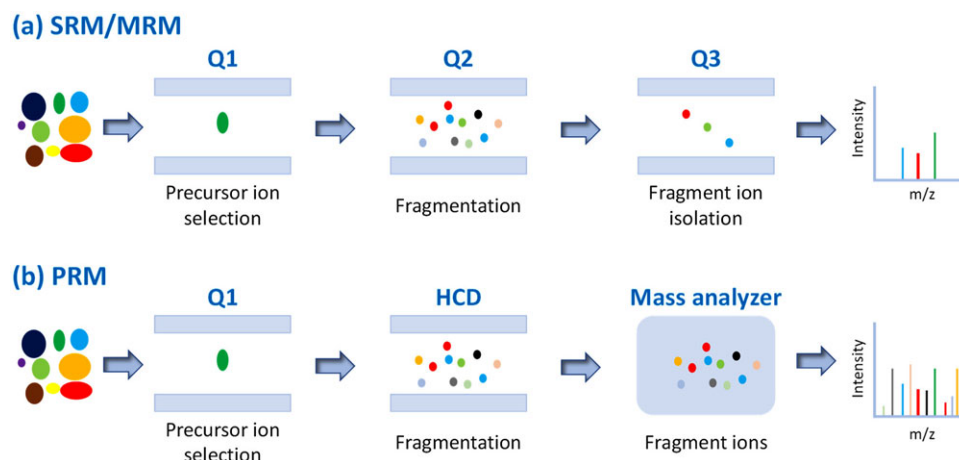
Figure 2. Schematic representation of targeted data acquisition approaches. a) SRM/MRM is typically performed on triple-quadrupole instruments where a predefined precursor ion is selected in the first quadrupole (Q1), fragmented in the second quadrupole (Q2) that serves as a collision cell and then specific fragment ions are monitored individually in the third quadrupole (Q3). b) PRM can be performed on quadrupole-orbitrap or QTOF instruments where Q1 selects the precursor ion that is then transferred to the higher energy collision-induced dissociation (HCD) cell for fragmentation. All fragment ions are then detected in the mass analyzer.
