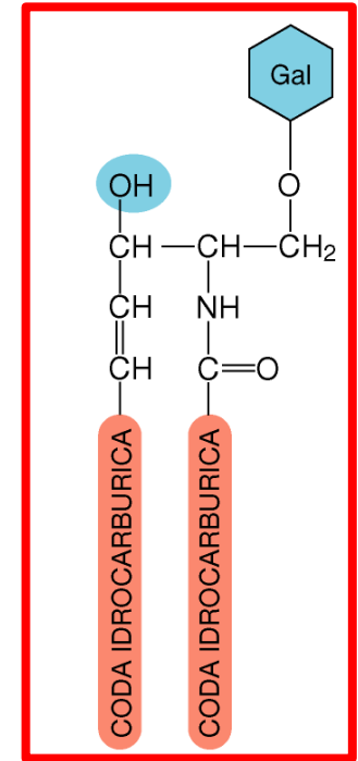
galattocerebroside (glicolipide)
