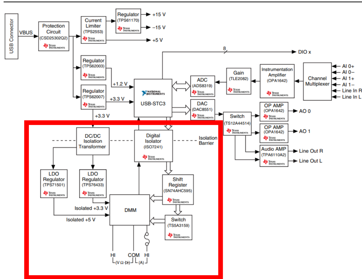
Figure 2. NI myDAQ Hardware Block Diagram
