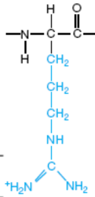
arginina
