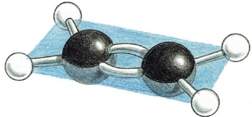
(B) etene
