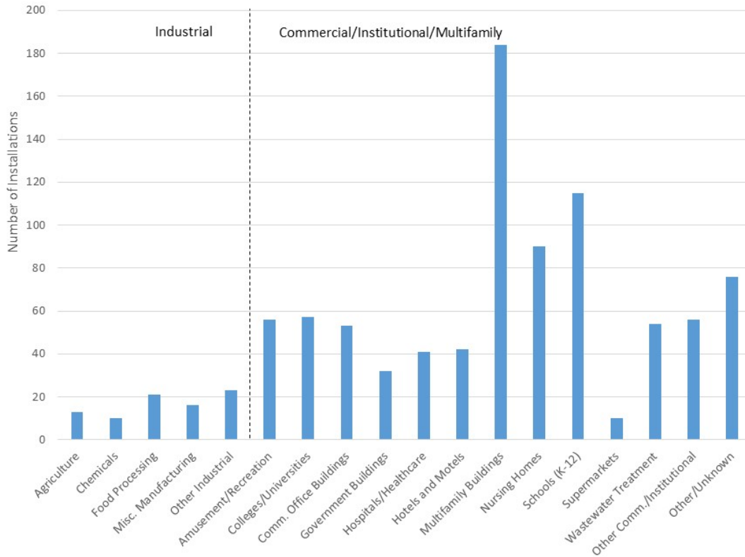
Figure 7-10. Packaged System Installations by Market Segment
