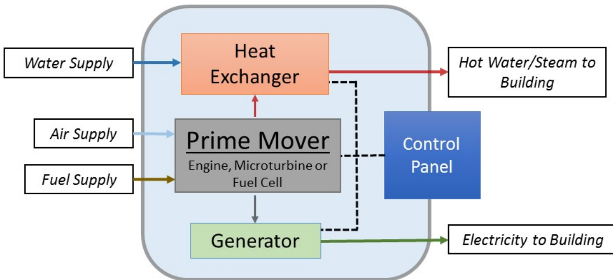
Figure 7-13. Packaged CHP System Diagram
