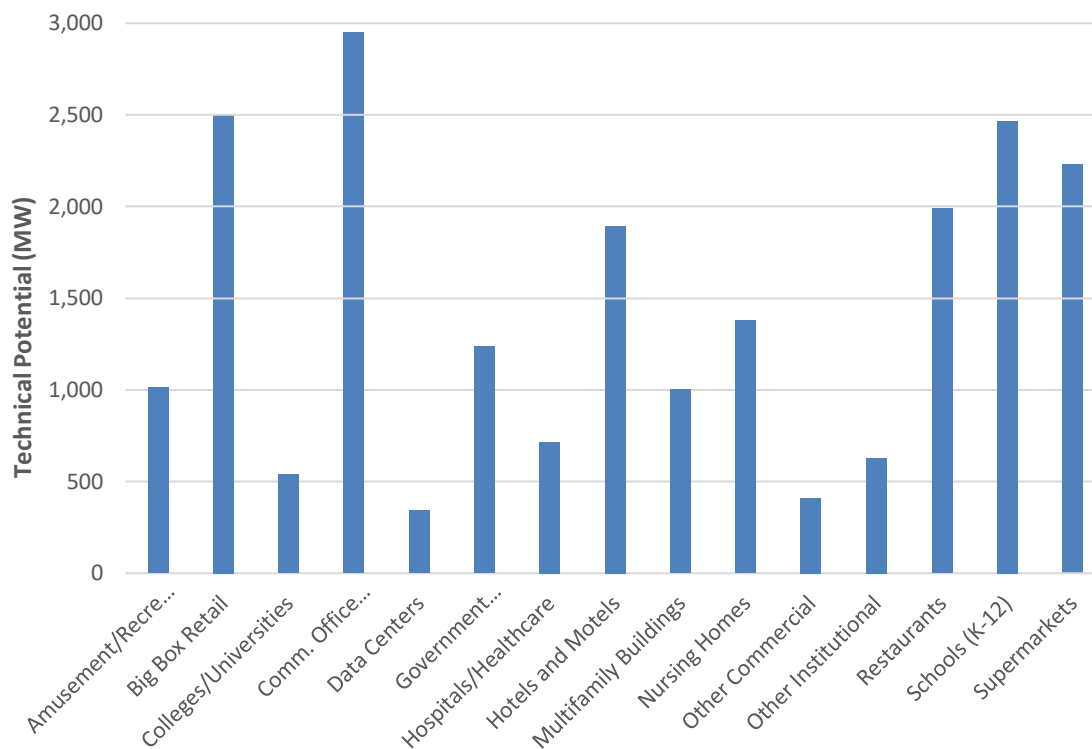
Figure 7-12. Technical Potential for <500 kW Packaged CHP Applications in the Commercial and Institutional Sectors, by Market Segment
