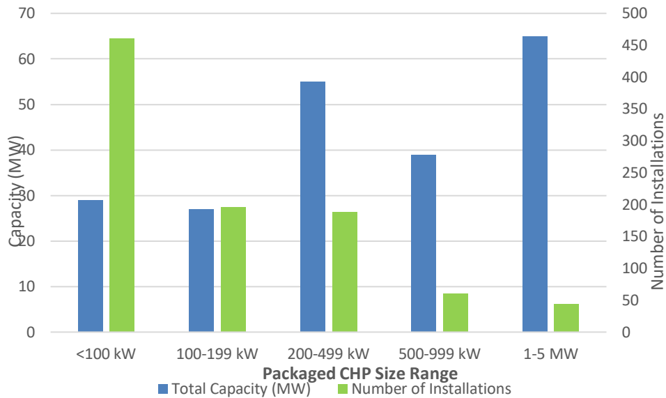
Figure 7-11. Packaged System Installations and Capacity by Size Range
